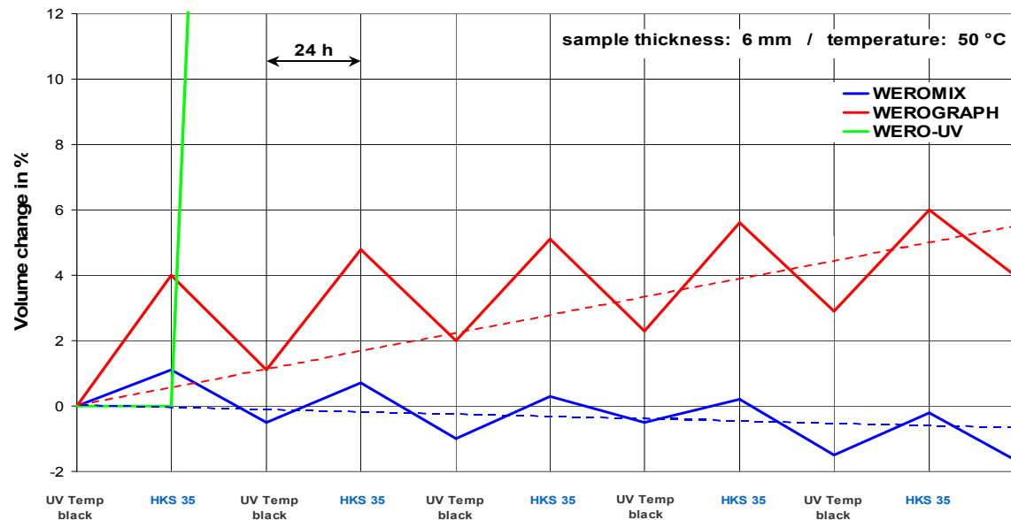
Swelling in UV and conventional ink
