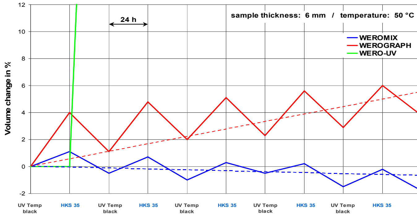
Swelling in UV and conventional ink
